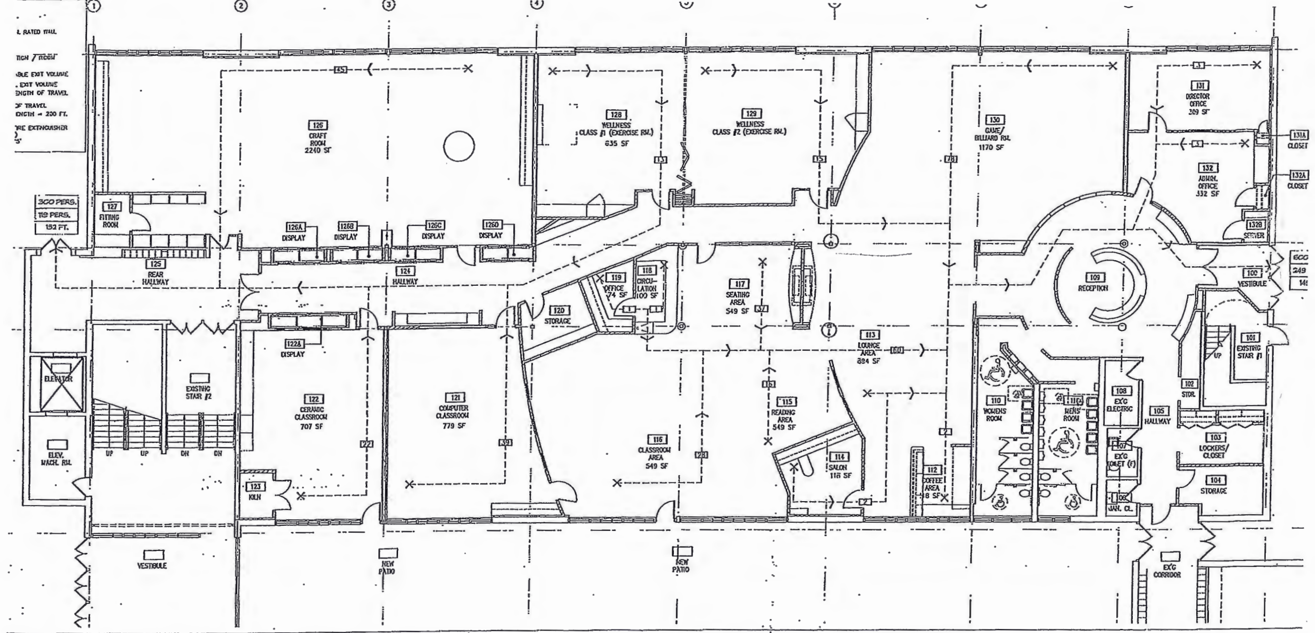
FIRST FLOOR EGRESS PLAN
